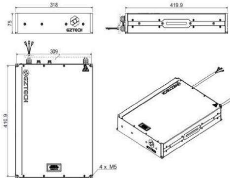
Laser dimension
