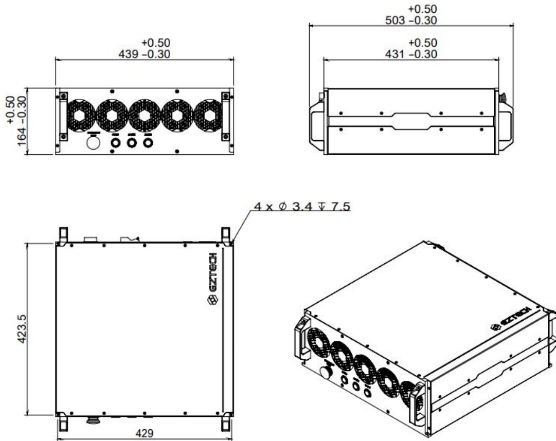
Laser dimension
