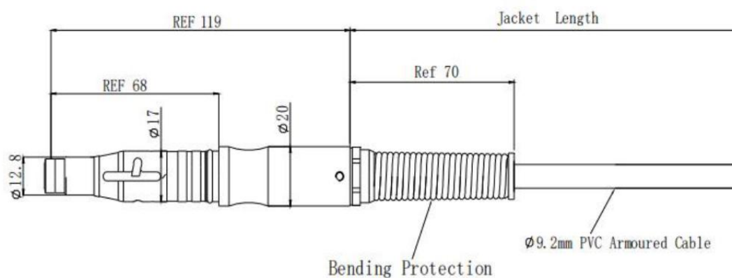
QBH dimension
