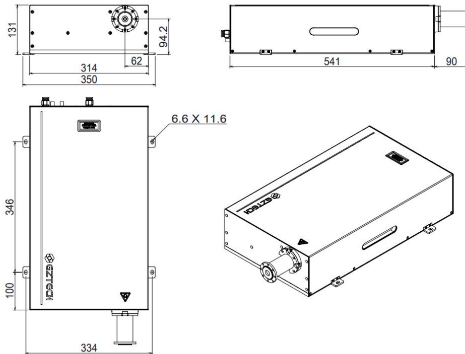
Laser dimension
